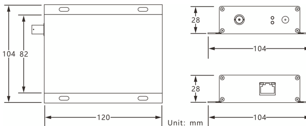
Receiver
