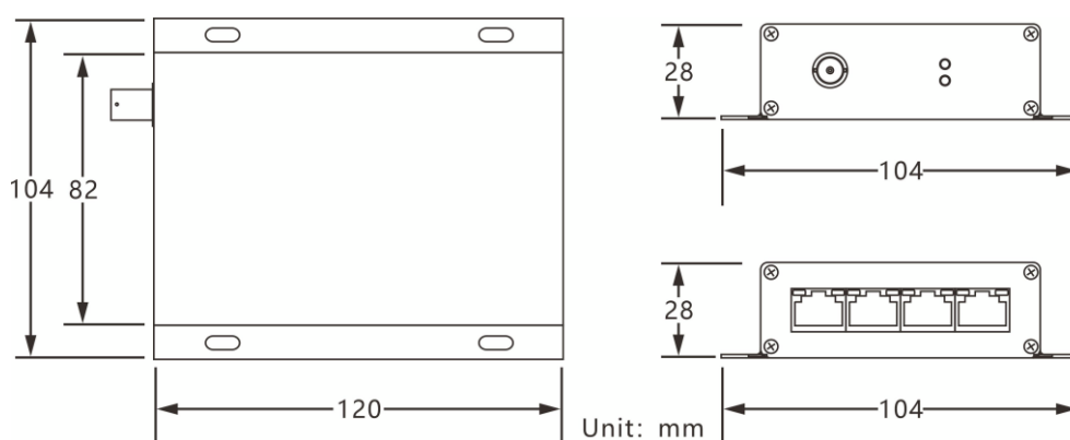
Transmitter
