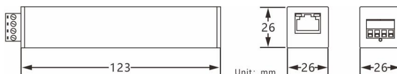
Transmitter Unit
