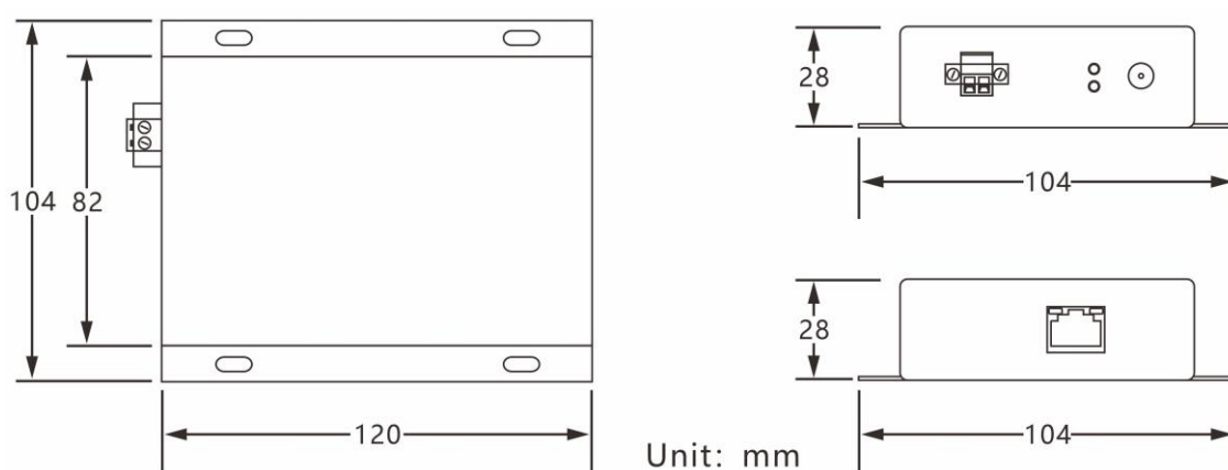
Receiver Unit
