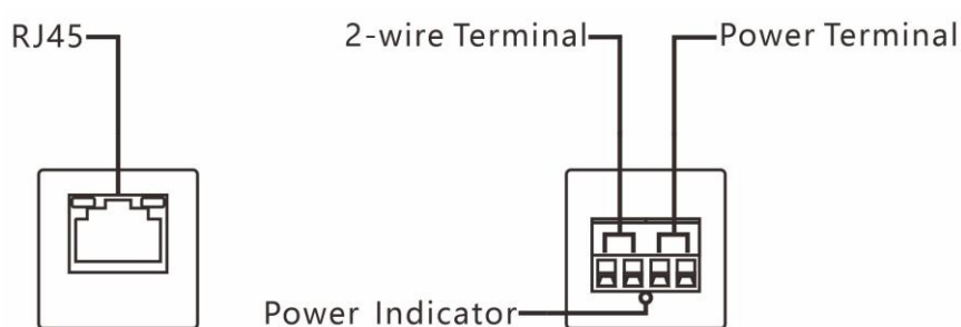
Transmitter Unit
